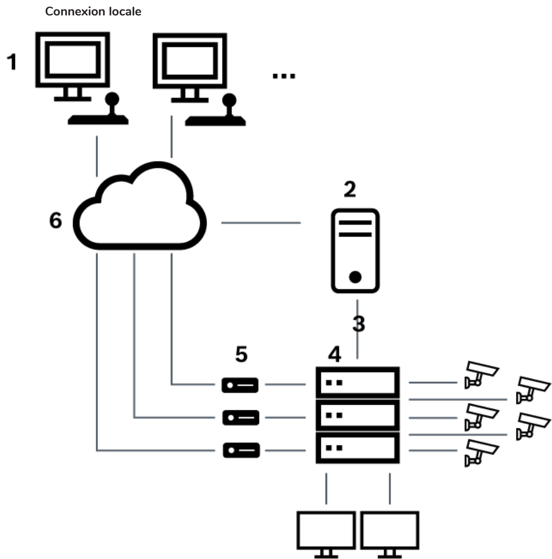
Figure 6.3: Connexion locale de Bosch Video Management System à la matrice Allegiant Bosch
